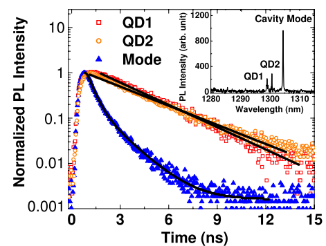
FIG. 1. (Color online) Time resolved experiments of the cavity mode and off-resonance QDs. Inset: spectrum of a L3 PhC cavity, under pulsed excitation ( \lambda=750 nm, average pump power P_{\text{av}}=0.4 \mu\text{W} in a 2 \mu\text{m} diameter spot), showing the cavity mode emission and two off-resonance excitonic lines from QDs. The fits of the experimental decays are shown in black.
